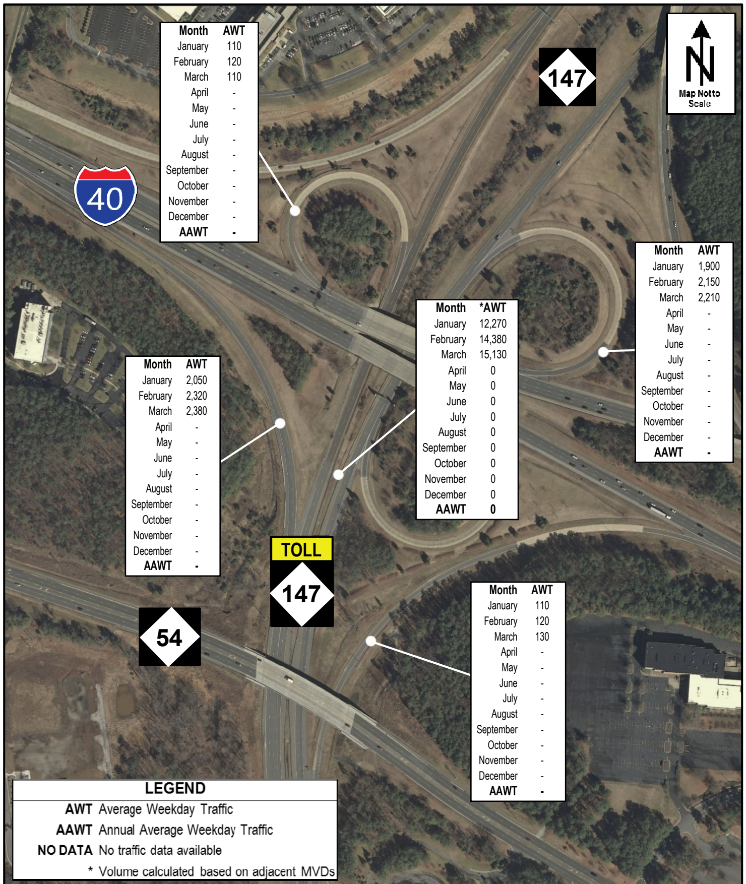
NC-147 at I-40 Interchange 2022 Average Weekday Traffic
