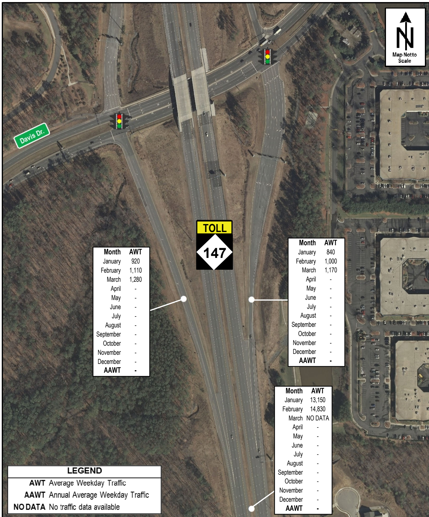
NC-147 at Davis Dr. Interchange 2022 Average Weekday Traffic
