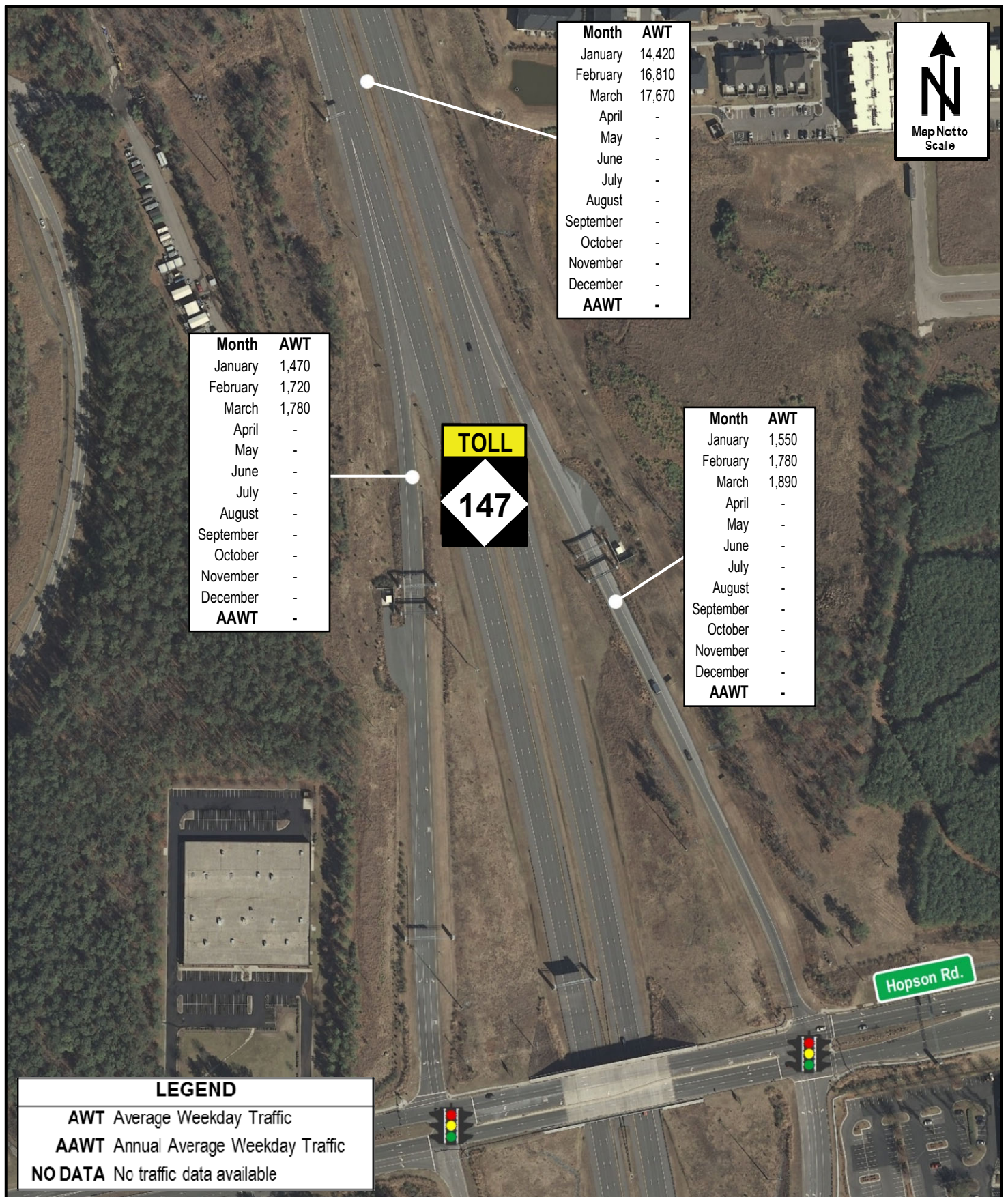
NC-147 at Hopson Rd. Interchange 2022 Average Weekday Traffic
