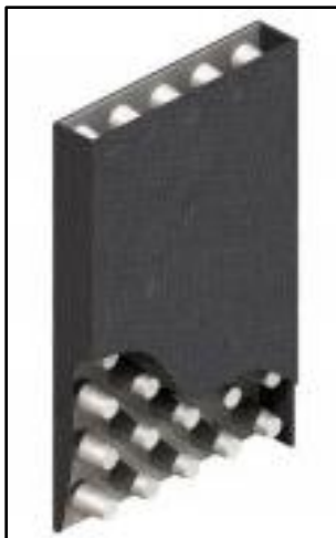
CAD drawing of vertical STRIP 9400 – image from American Wick Drain brochure
